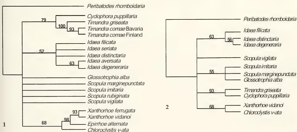
Fig. 1. Bootstrap 50% majority-rule consensus tree for 19 Geometrid taxa using 135 informative sites of the mitochondrial ND1 gene (rooted with Peribatodes rhomboidaria ). Settings for tree computation: Heuristic search, bootstrap with 100 replicates.
